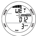
Fig. 32 - NORM SURFACE MAIN (Post Dive Wet)
