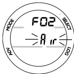
Fig. 37 - SET FO2 (Air setting)
